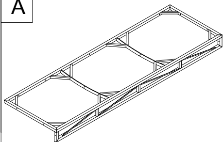
Seat Chair Frame (1 pc)
